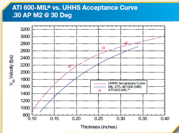
Typical ballistic results of ATI 600-MIL® against 30 Cal. AP M2 projectile. (Courtesy of Army Research Labs).
