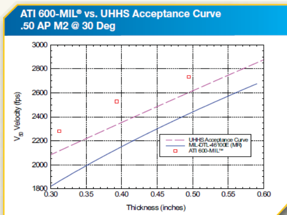
Typical ballistic results of ATI 600-MIL® against 50 Cal. AP M2 projectile. (Courtesy of Army Research Labs).
